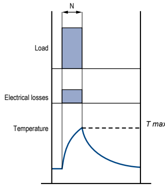
Fig. 2. - Short-time duty. Type S2.
